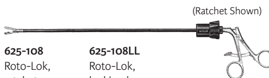
610-108 Roto-Lok, slide lock, insulated shaft, 5mm, 326mm
