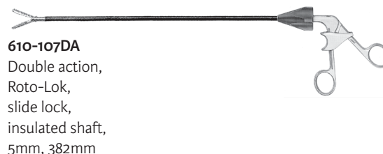
610-107 Roto-Lok, slide-lock, insulated shaft, 5mm, 381mm
